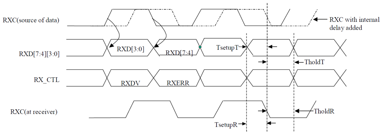
Figure 5-46. RGMII Interface Receive Timing
