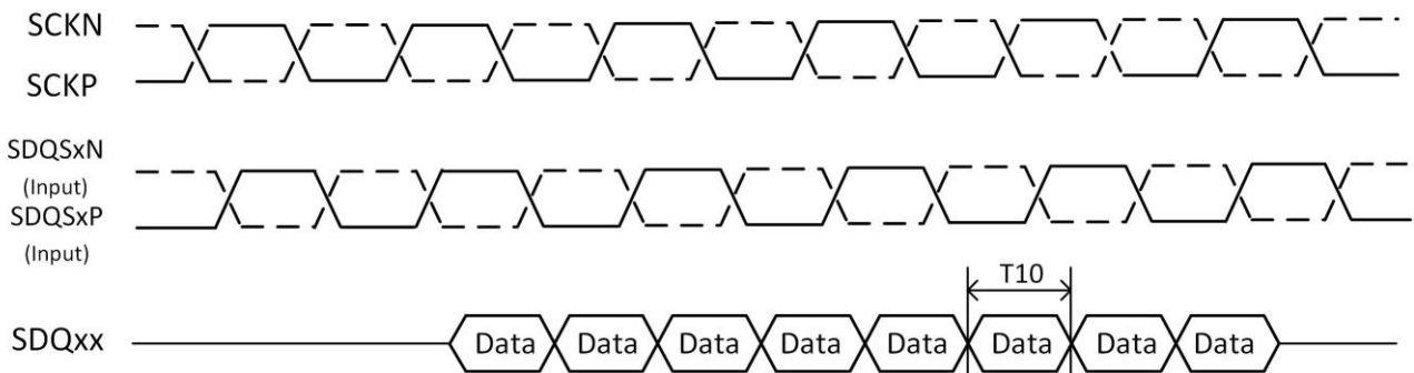
Figure 5-13. DDR4 Read Cycle
