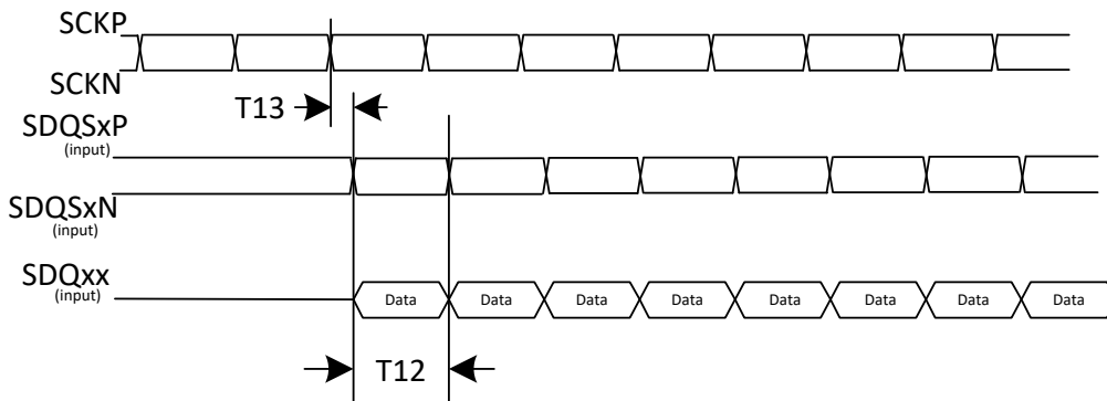
Figure 5-7. DDR3/DDR3L Read Cycle
