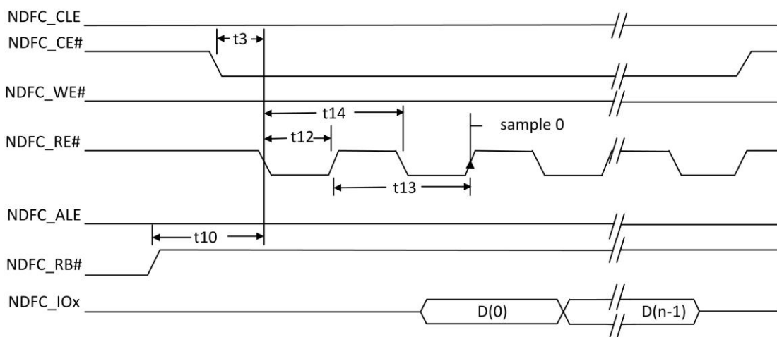
Figure 5-19. Extending EDO Type Serial Access Mode Timing (SAM2)
