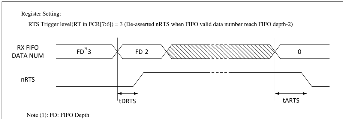
Figure 5-52. UART nRTS Timing
