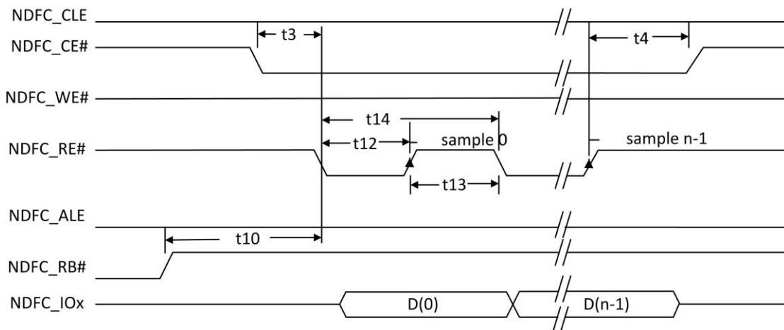
Figure 5-17. Conventional Serial Access Cycle Timing (SAM0)
