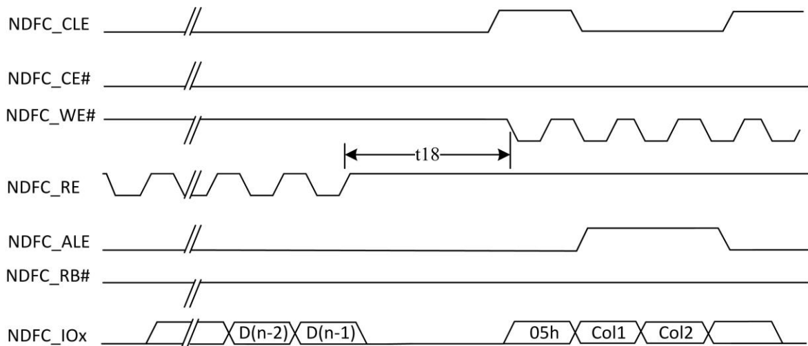
Figure 5-25. RE# High to WE# Low Timing
