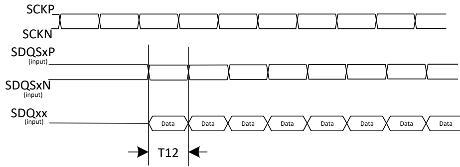
Figure 5-4. LPDDR2 Read Cycle
