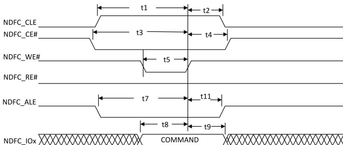
Figure 5-20. Command Latch Cycle Timing
