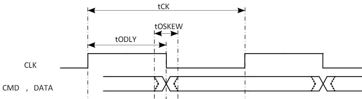
Figure 5-33. SMHC2 HS-SDR Mode Output Timing Diagram
