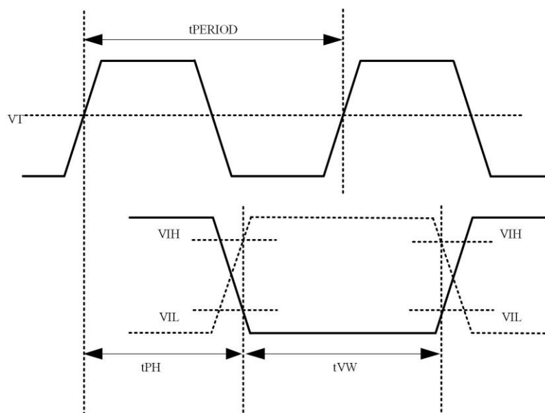
Figure 5-38. SMHC2 HS200 Mode Input Timing Diagram
