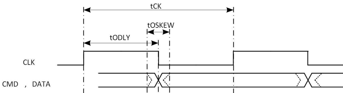
Figure 5-31. SMHC0/1 SDR104 Mode Output Timing Diagram
