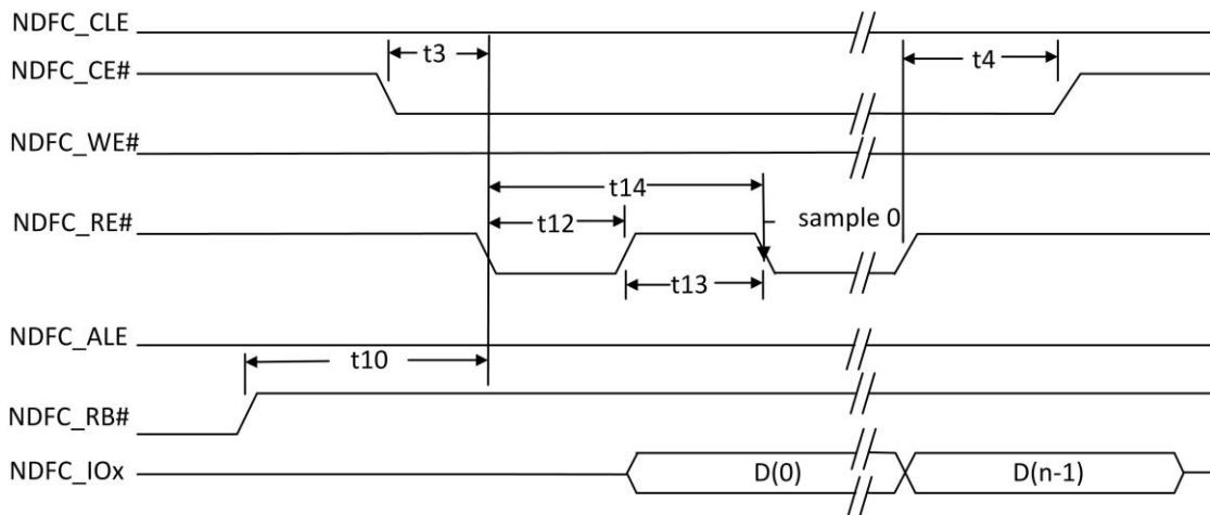
Figure 5-18. EDO Type Serial Access after Read Cycle Timing (SAM1)
