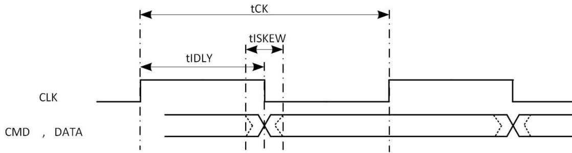
Figure 5-28. SMHC0/1 SDR Mode Input Timing Diagram
