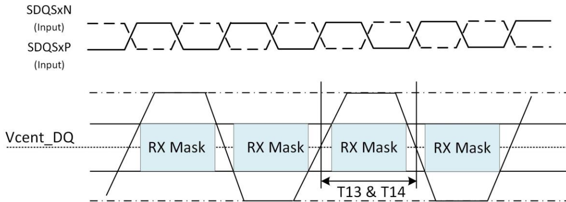
Figure 5-16. LPDDR4 Read Cycle
