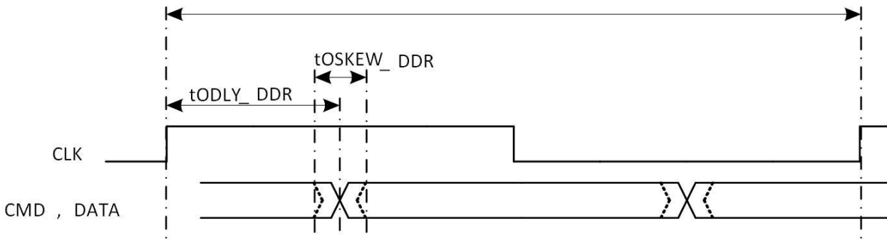
Figure 5-34. SMHC2 HS-DDR Mode Output Timing Diagram
