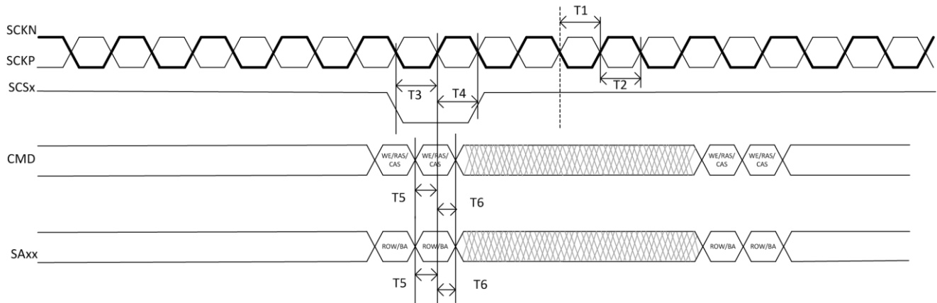
Figure 5-8. LPDDR3 Command and Address Timing Diagram
