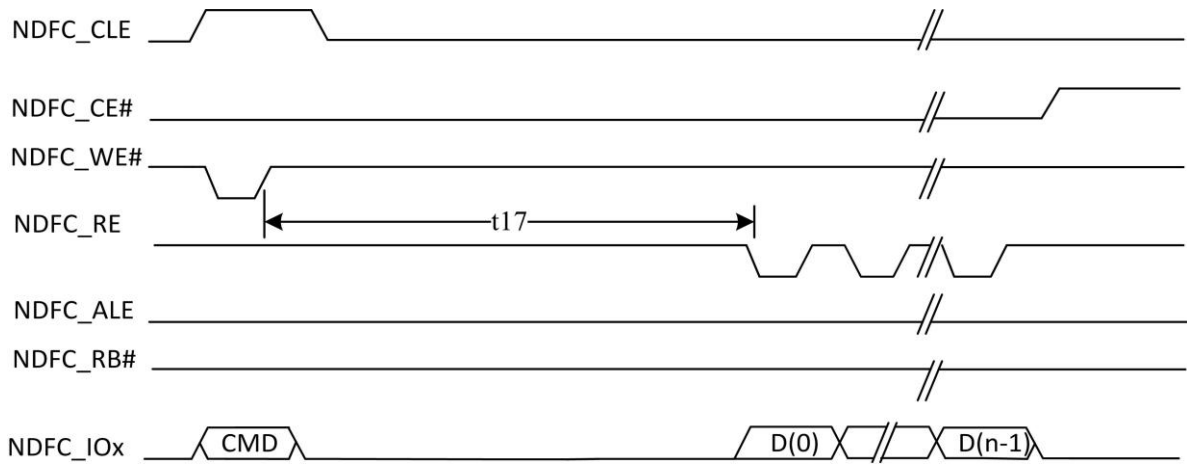
Figure 5-24. WE# High to RE# Low Timing
