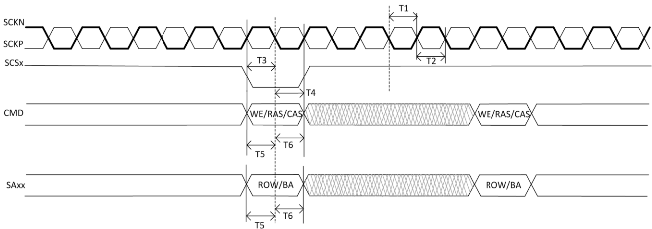
Figure 5-5. DDR3/DDR3L Command and Address Timing
