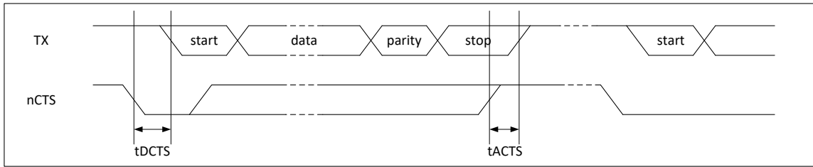
Figure 5-51. UART nCTS Timing
