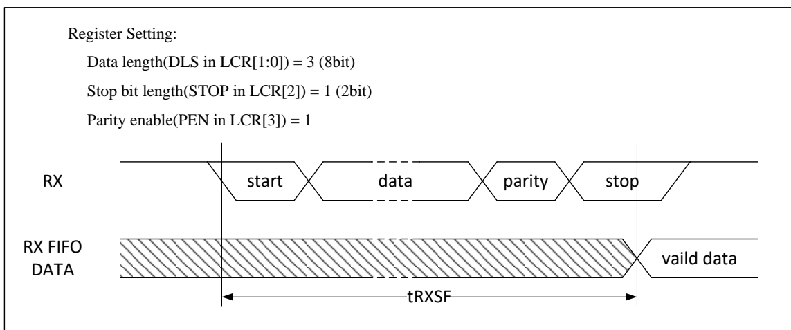
Figure 5-50. UART RX Timing
