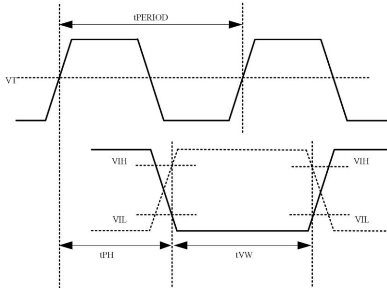
Figure 5-32. SMHC0/1 SDR104 Mode Input Timing Diagram
