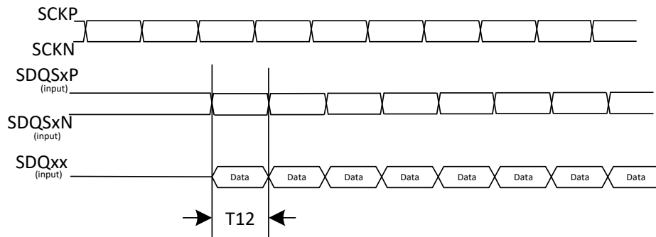
Figure 5-10. LPDDR3 Read Cycle
