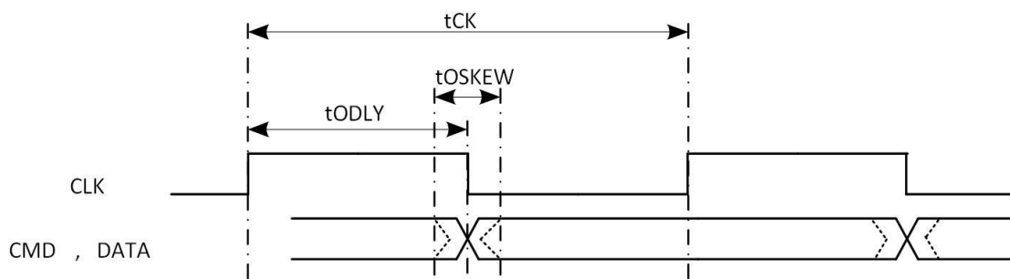
Figure 5-27. SMHC0/1 SDR Mode Output Timing Diagram
