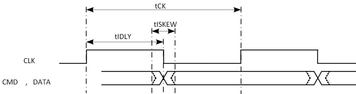
Figure 5-35. SMHC2 HS-SDR Mode Input Timing Diagram
