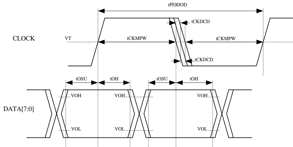
Figure 5-39. SMHC2 HS400 Mode Data Output Timing Diagram
