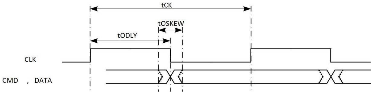
Figure 5-37. SMHC2 HS200 Mode Output Timing Diagram
