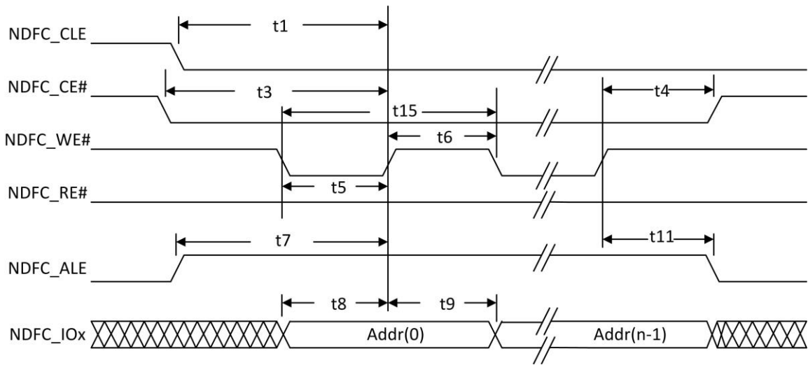
Figure 5-21. Address Latch Cycle Timing
