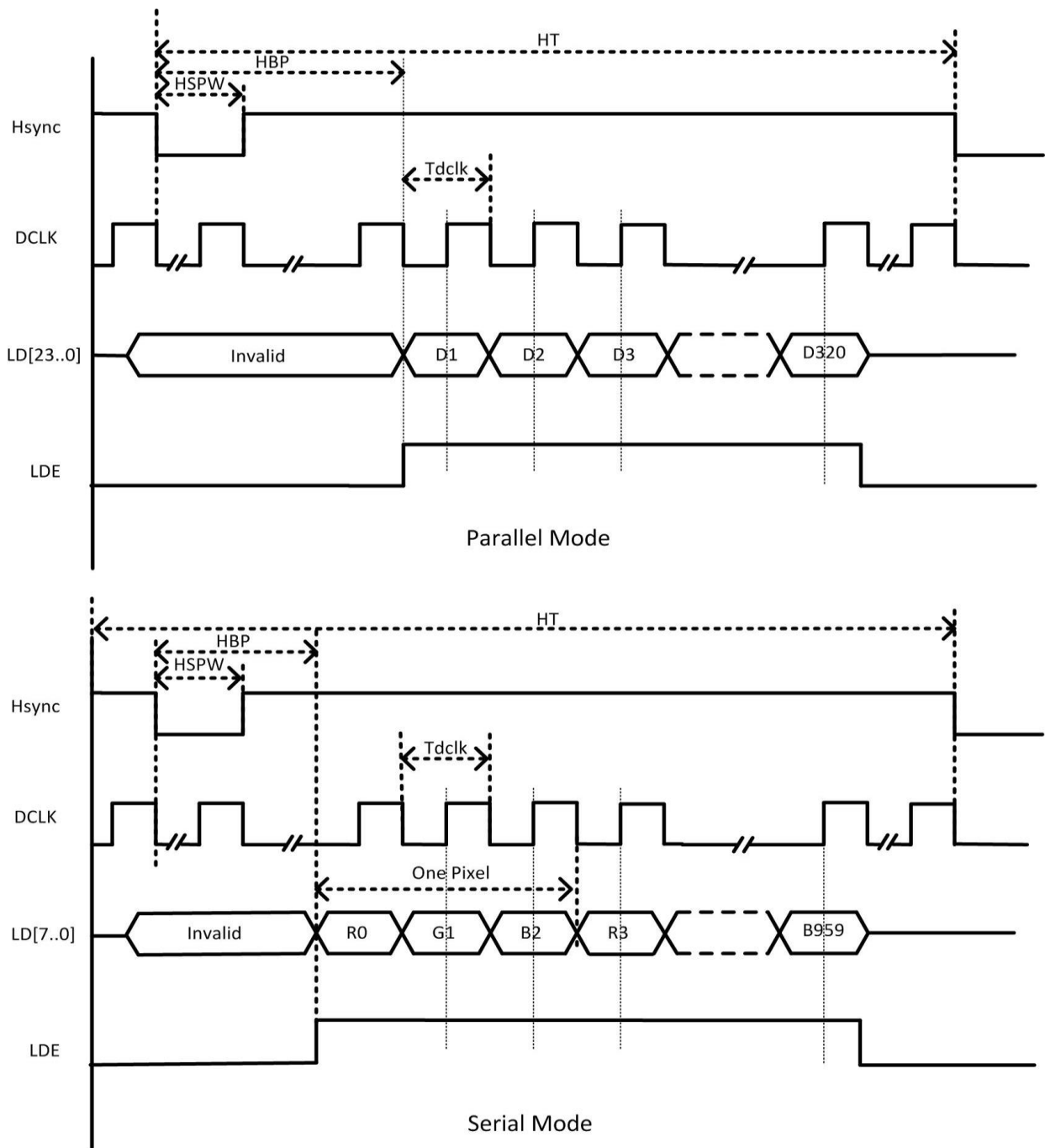
Figure 5-42. HV_IF Interface Horizontal Timing
