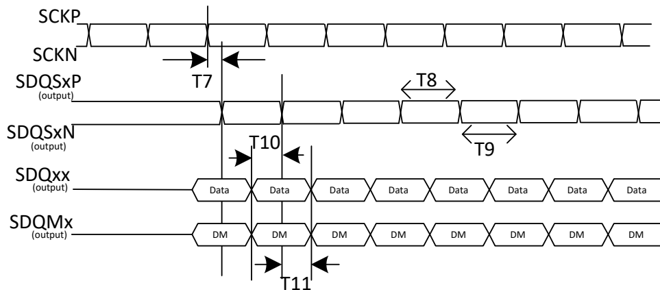
Figure 5-9. LPDDR3 Write Cycle
