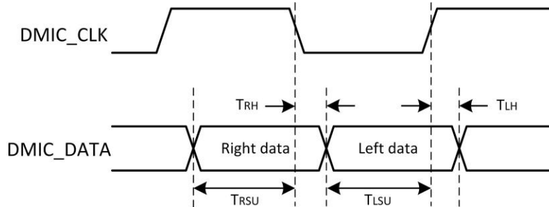
Figure 5-56. DMIC Timing
