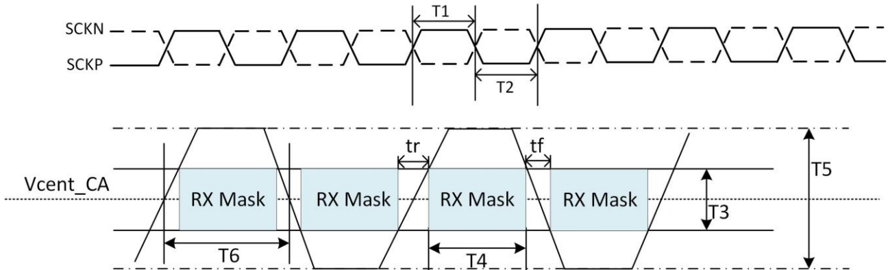
Figure 5-14. LPDDR4 Command and Address Timing Diagram
