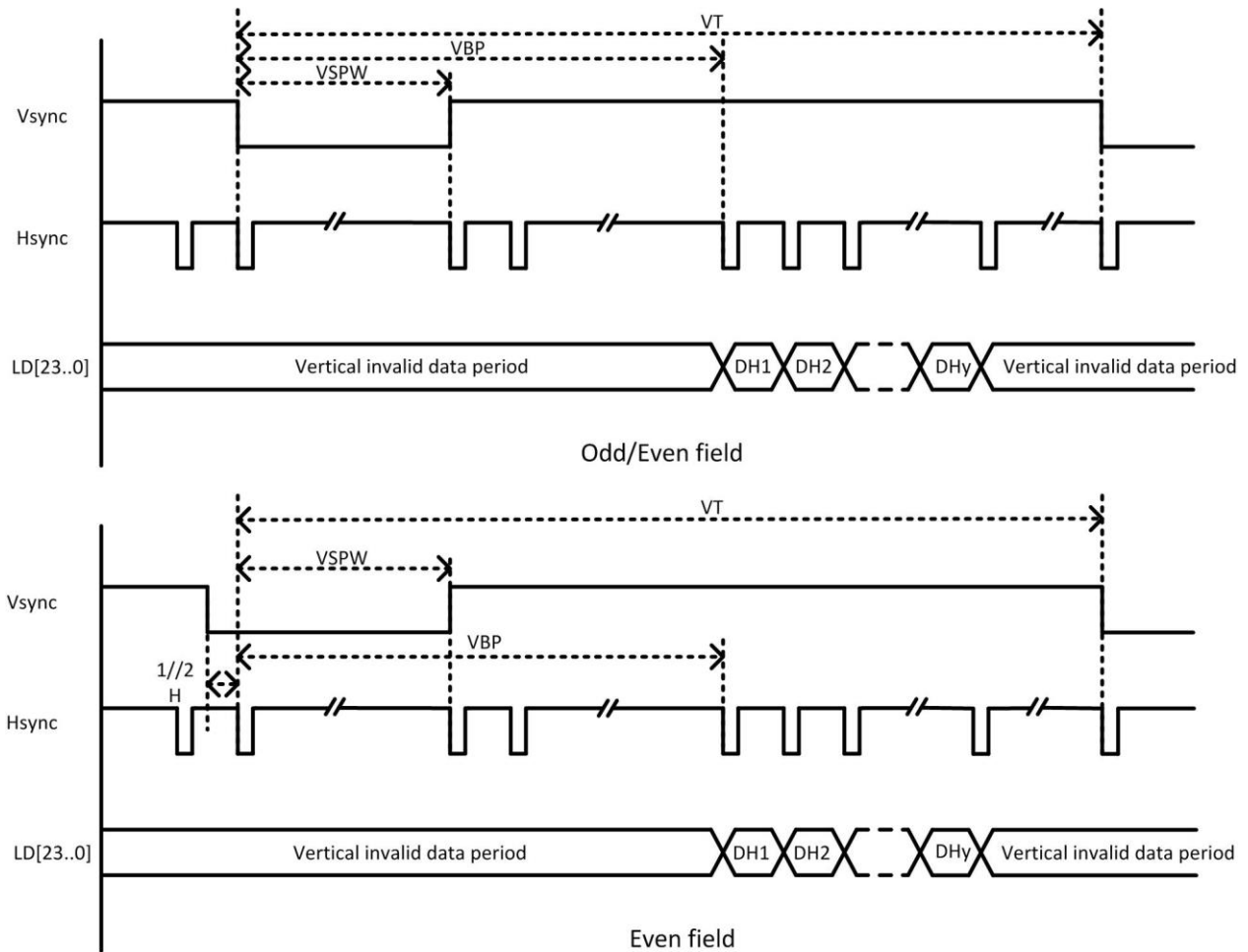
Figure 5-41. HV_IF Interface Vertical Timing
