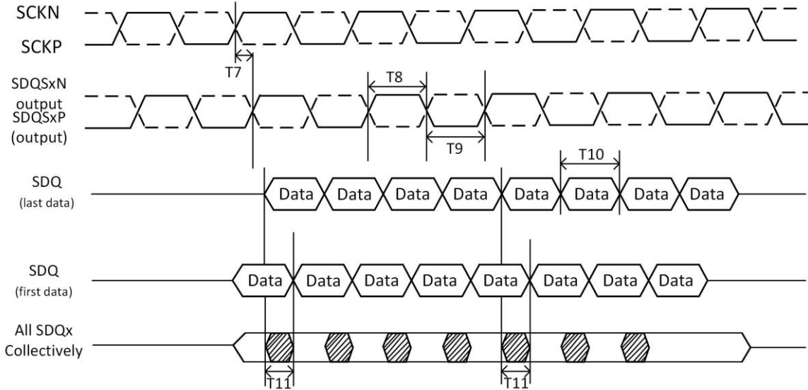
Figure 5-12. DDR4 Write Cycle
