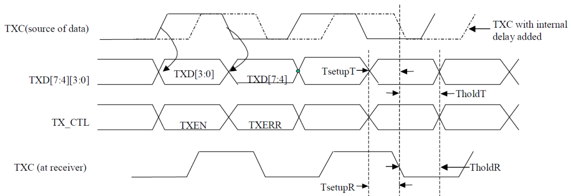
Figure 5-45. RGMII Interface Transmit Timing
