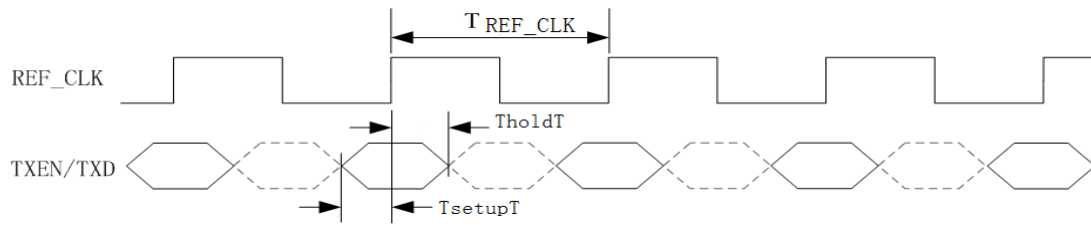
Figure 5-43. RMII Interface Transmit Timing
