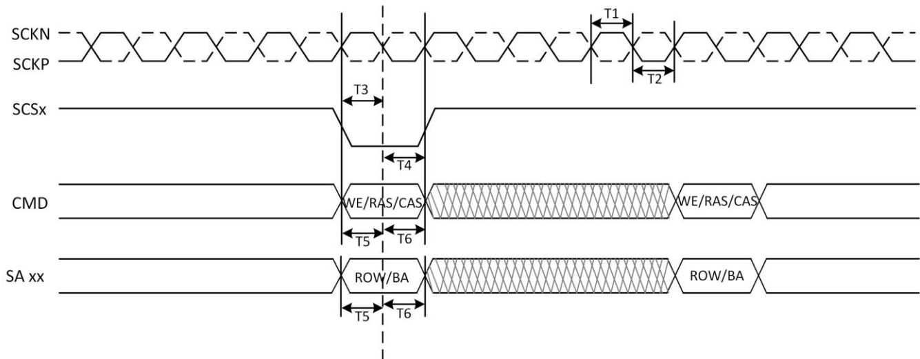
Figure 5-11. DDR4 Command and Address Timing
