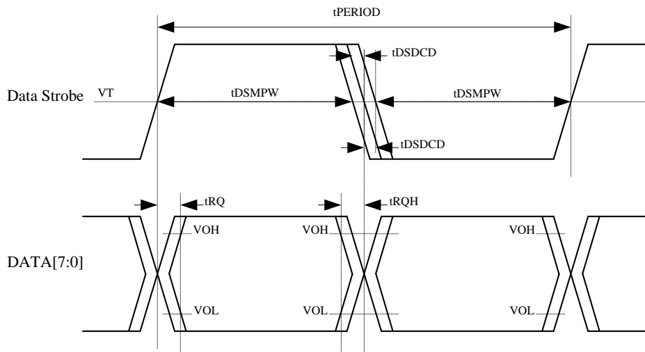
Figure 5-40. SMHC2 HS400 Mode Data Input Timing Diagram
