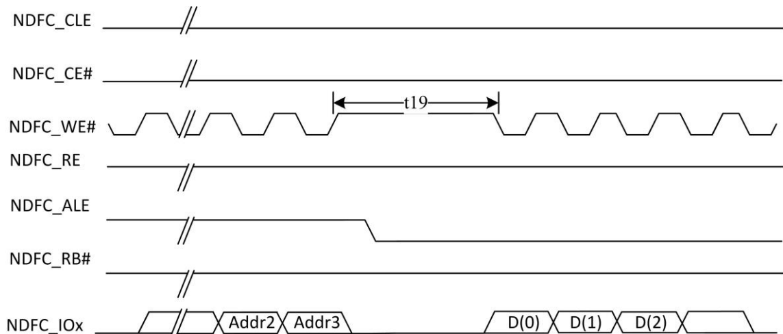
Figure 5-26. Address to Data Loading Timing
