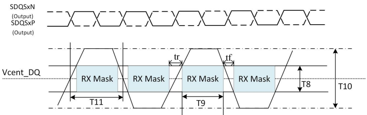
Figure 5-15. LPDDR4 Write Cycle
