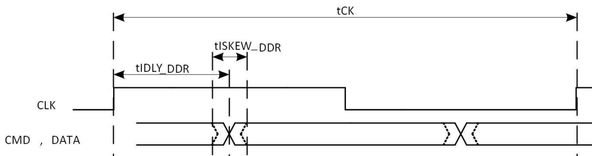
Figure 5-36. SMHC2 HS-DDR Mode Input Timing Diagram
