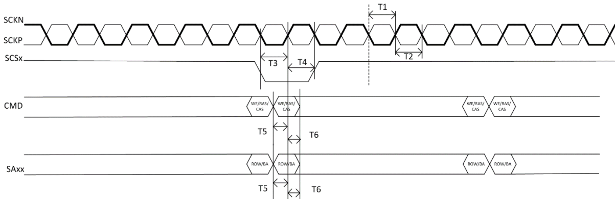
Figure 5-2. LPDDR2 Command and Address Timing Diagram
