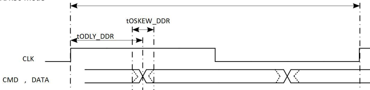
Figure 5-29. SMHC0/1 DDR50 Mode Output Timing Diagram
