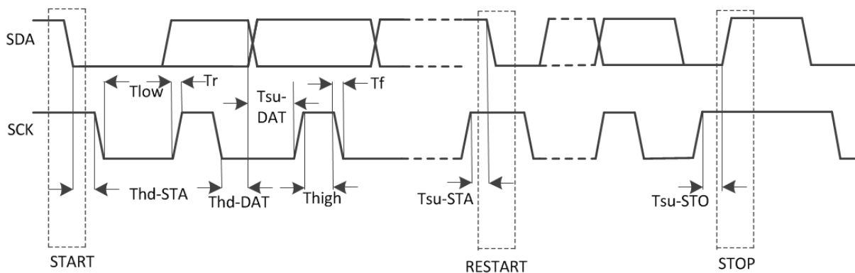
Figure 5-53. TWI Timing
