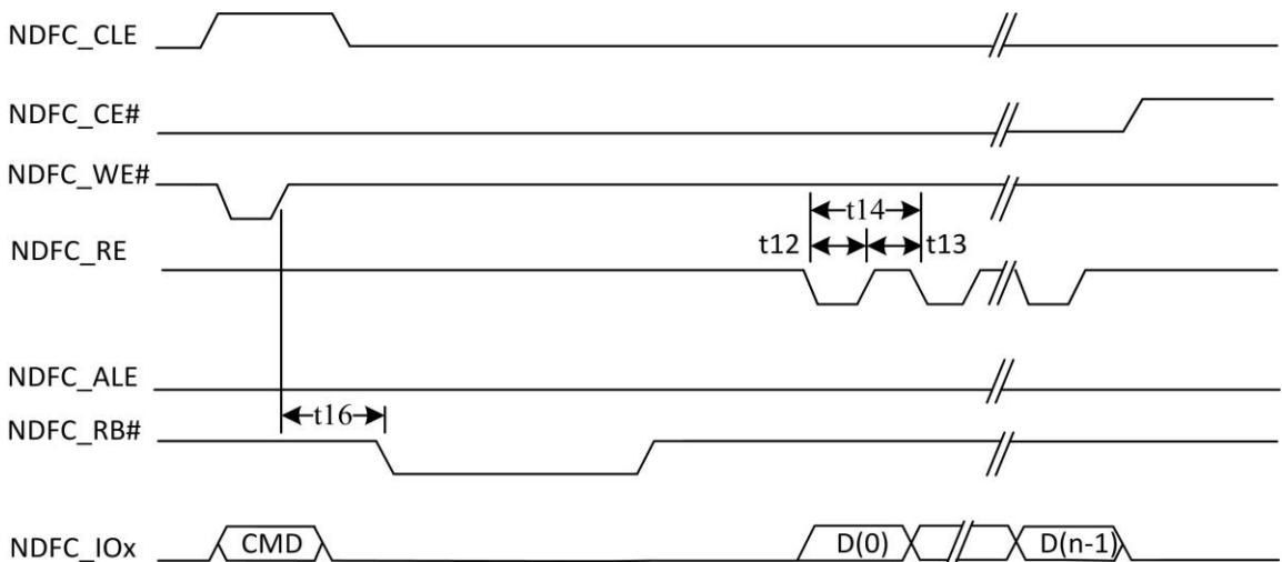
Figure 5-23. Waiting R/B# Ready Timing
