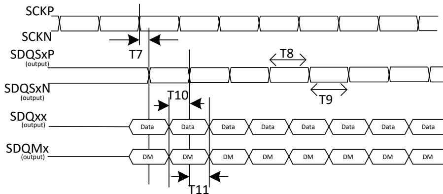
Figure 5-3. LPDDR2 Write Cycle
