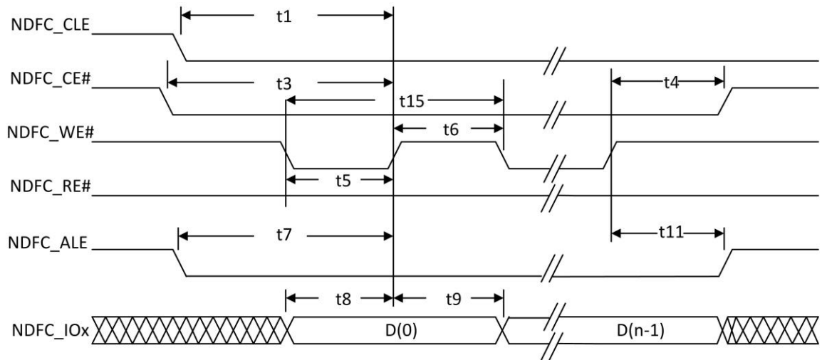
Figure 5-22. Write Data to Flash Cycle Timing
