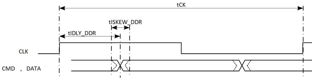
Figure 5-30. SMHC0/1 DDR50 Mode Input Timing Diagram
