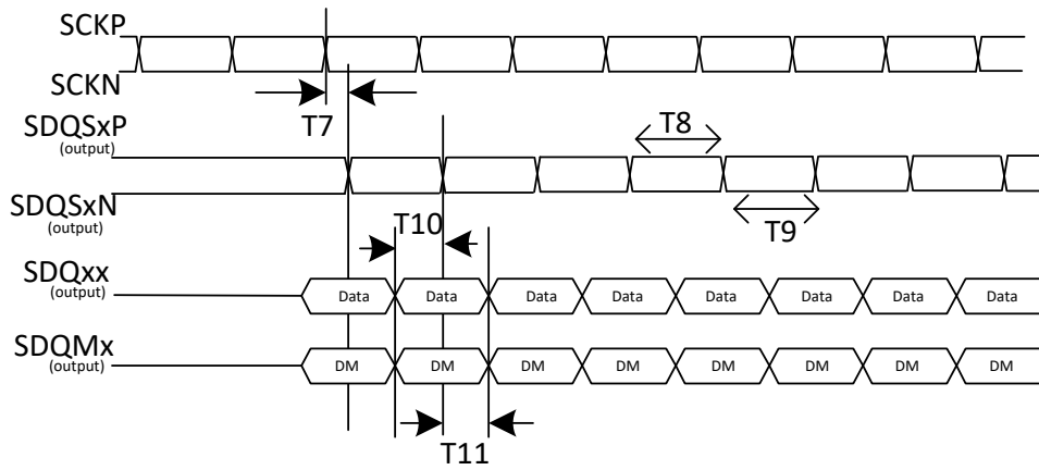
Figure 5-6. DDR3/DDR3L Write Cycle
